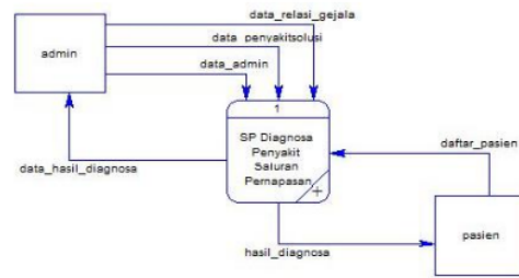
Gambar 2 Context Diagram
