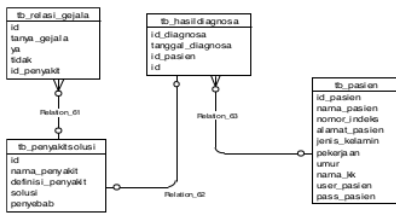
Gambar 8 Conceptual Data Model
