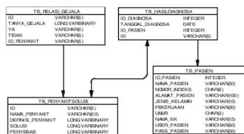
Gambar 9 Physical Data Model
