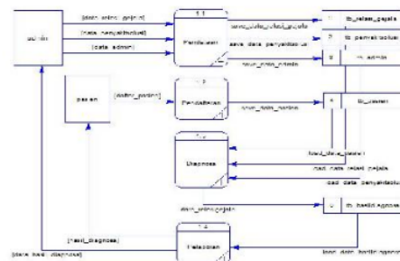
Gambar 3 Data Flow Diagram
