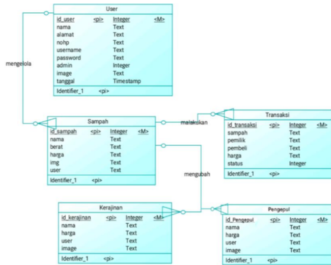
Gambar 4 CDM (Conceptual Data Model)
