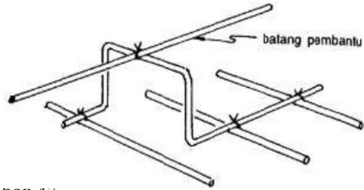
Gambar 47 Support Tradisional
